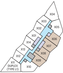
LEVEL 26, 28, 30, 32, 34 TYPICAL FLOOR PLAN
