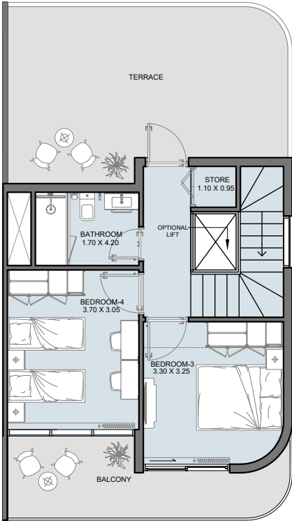
SECOND FLOOR Corner Unit
