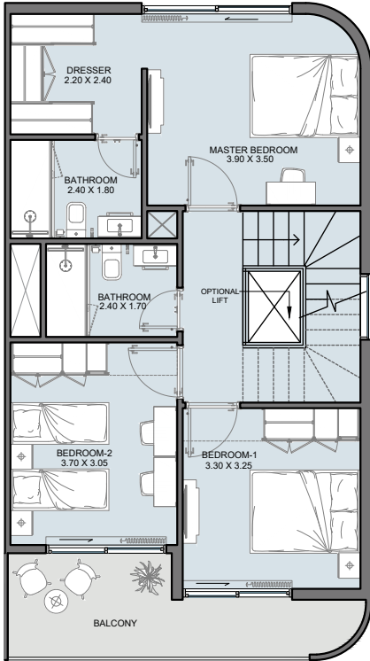
FIRST FLOOR Corner Unit
