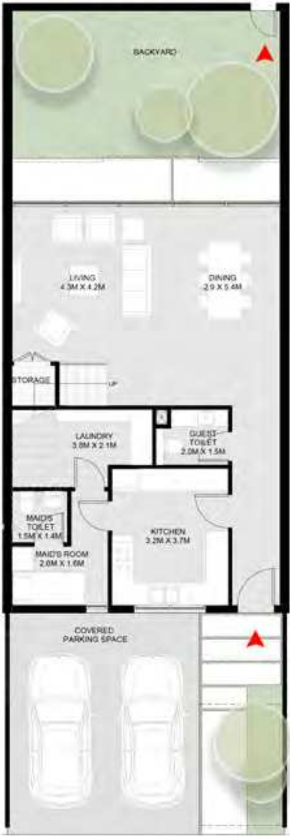
Ground Floor
