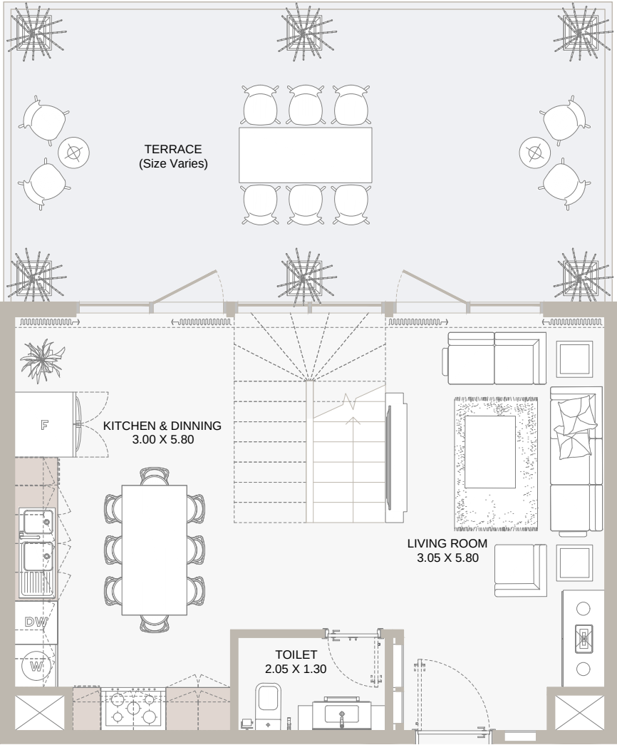
Ground Level
