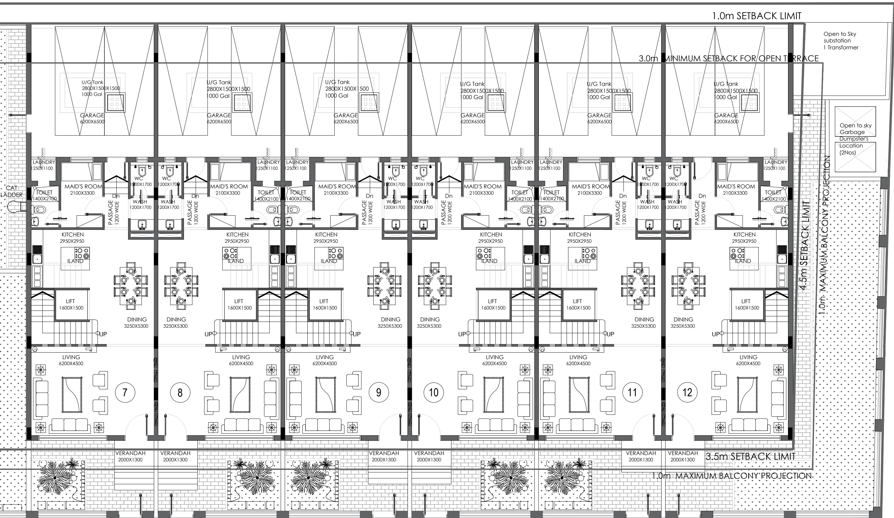
GROUND FLOOR
