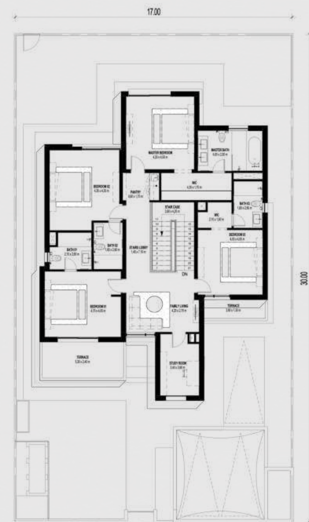
FIRST FLOOR
