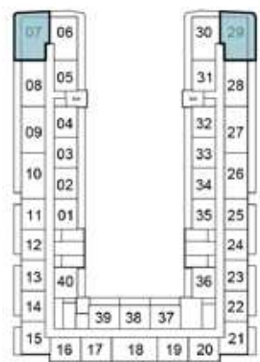
2ND FLOOR
